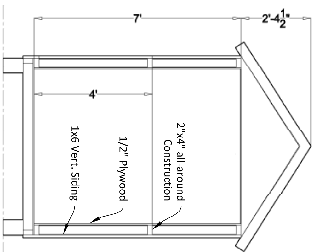
Cross-section A-A
